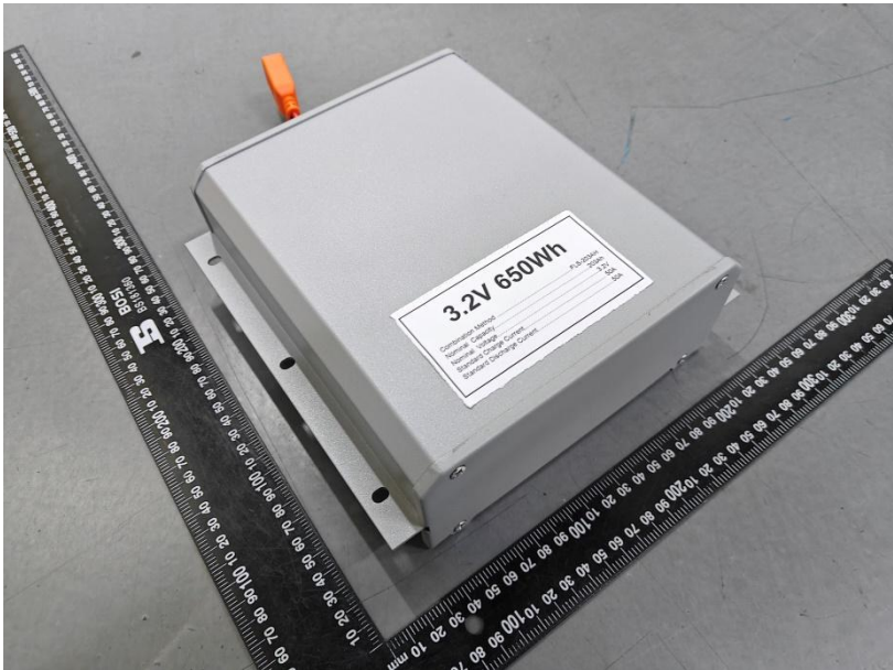
Cell: FLS-203AH, 3.2V, 203Ah, 650Wh
